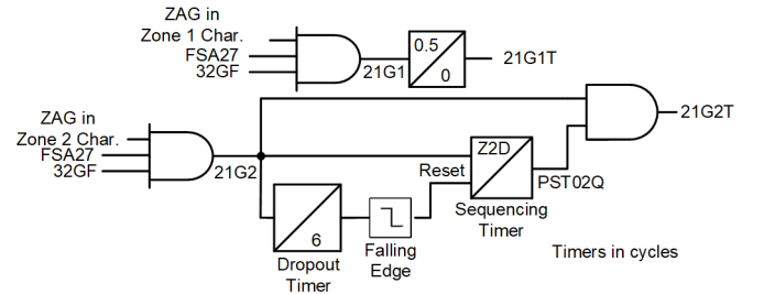
Fig. 13. Distance zone timer example
