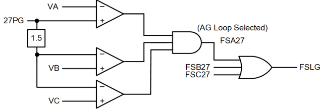
Fig. 11. Voltage-based FIDS logic for ground loop selection
