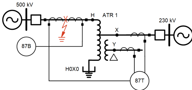
Fig. 23. Field case study, fault in the overlapping of the autotransformer differential (87T) and the busbar differential (87B).
