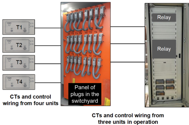
Fig. 29. Panel of plugs showing autotransformer units T1, T2, and T4 selected as phases A, B, and C, respectively, T3 selected as spare unit (not in scale).
