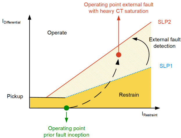
Fig. 21. Adaptive percentage restrained differential characteristic.
