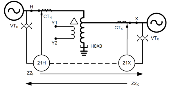
Fig. 11. Overreaching distance elements applied with a directional comparison scheme to detect internal faults in an autotransformer.
