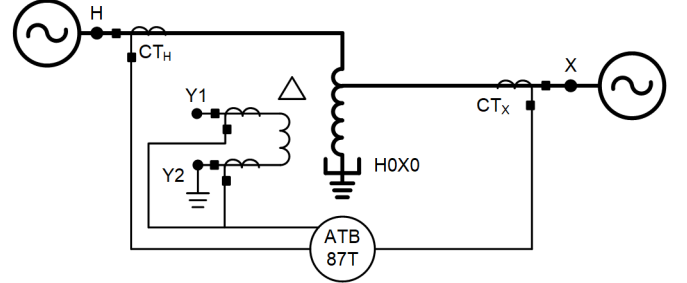
Fig. 8. ATB differential element with CTs available at both sides of the tertiary winding.
