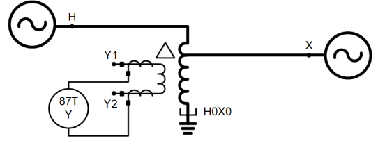
Fig. 10. Delta-dedicated differential element when CTs are available at both sides of the tertiary winding.
