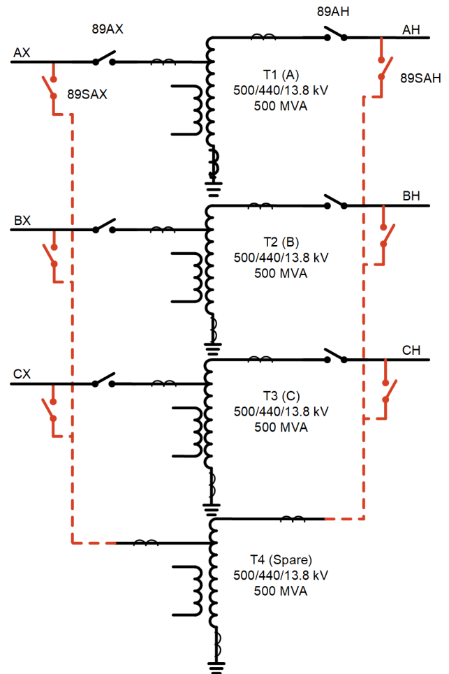
Fig. 28. A three-line diagram of an installation with a designated spare autotransformer with motorized disconnecting switches for unit replacement (tertiary buswork not shown for simplicity).
