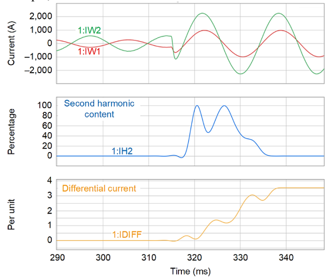
Fig. 22 shows that the second harmonic content takes about one cycle (16.67 millisecond) to reach zero after the rise of the differential current.
