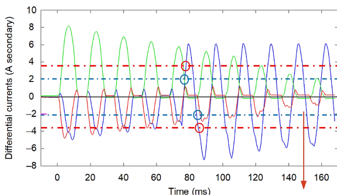
Fig. 25. Differential currents for an internal fault during transformer energization.
