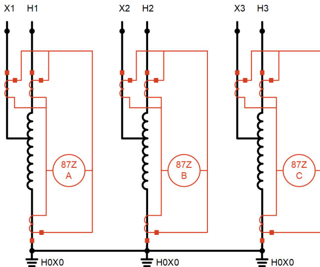
Fig. 20. Three-phase high-impedance differential element scheme (tertiary winding not shown for simplicity).
