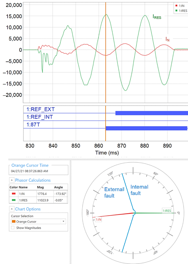
Fig. 16. Field case study-event report for the fault in the H side of ATR 1.
