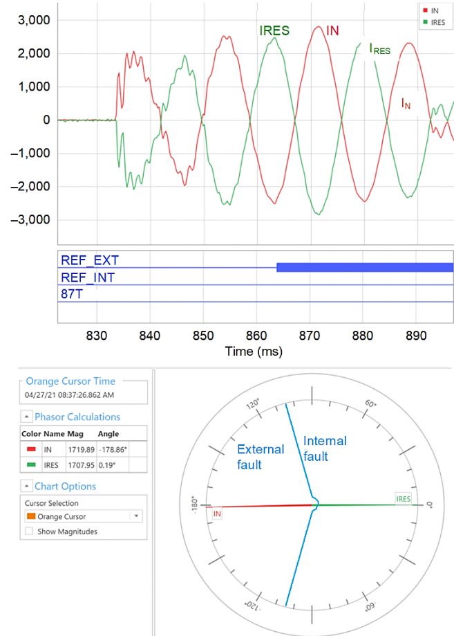
Fig. 17. Field case study-event report from the ATR 2 protection system for the fault in the H side of ATR 1.
