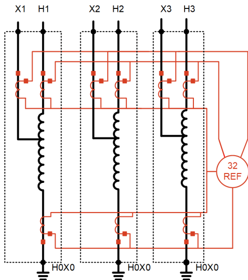
Fig. 19. Directional-based REF applied to an autotransformer bank with a single neutral CT.
