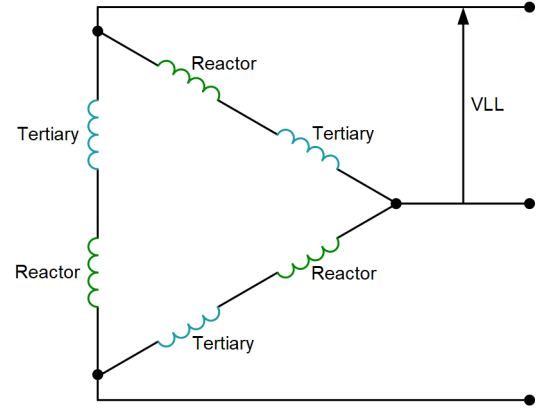
Fig. 2. Example of a tertiary autotransformer winding connection, with a high-reactance reactor connected inside the delta.
