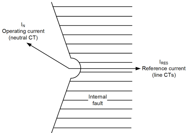
Fig. 12. Characteristic of operation of directional-based REF element.
