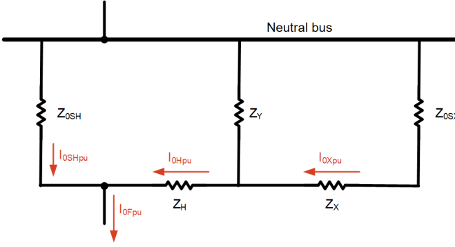
Fig. 14. Autotransformer zero-sequence network for an SLG fault in the high-voltage side.
