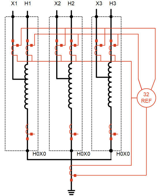
Fig. 18. Not recommended application of directional-based REF using residual connection of H0X0 bushing CTs.
