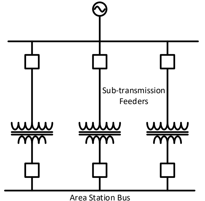
Fig. 1. High level arrangement of an area substation
