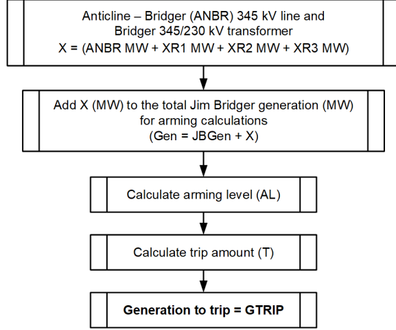
Fig. 3. Arming level and generation to shed calculation flow chart.
