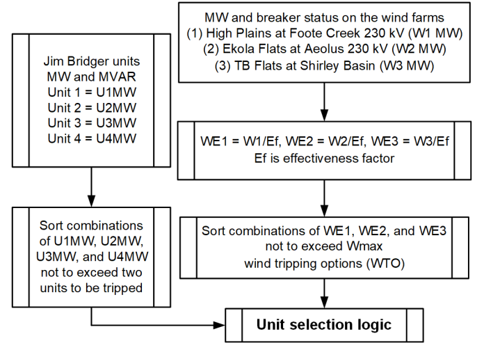
Fig. 4. Inputs to unit selection logic.
