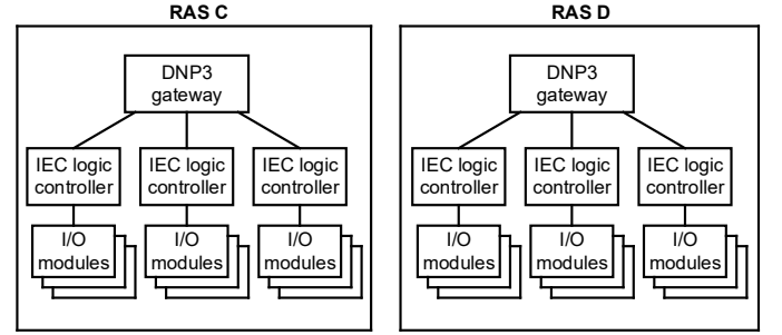
Fig. 11. Dual TMR architecture.
