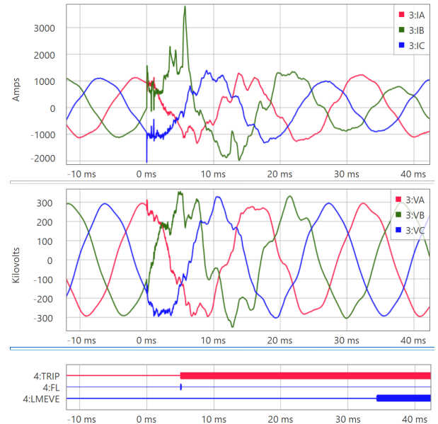
Fig. 54. West Shackelford currents and voltages and line monitor event.
