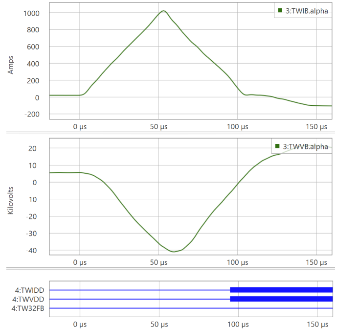
Fig. 48. West Shackleford B-phase alpha-mode current and voltage TWs and digital bits.
