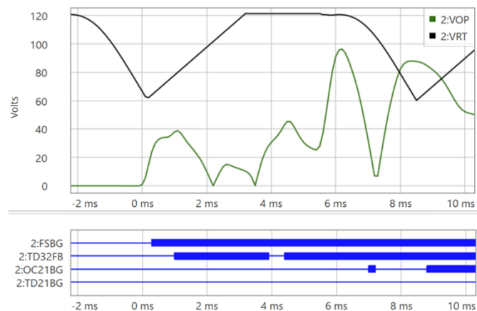
Fig. 47. West Shackleford TD21BG restrains.
