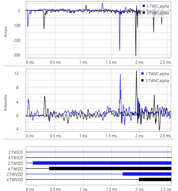
Fig. 24. West Shackelford (blue) and Sam (black) C-phase alpha-mode current and voltage TWs and digital bits operating times.
