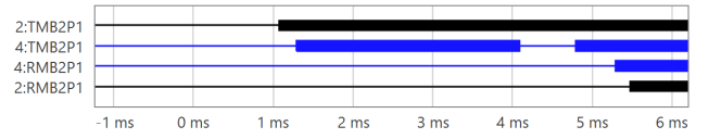
Fig. 52. POTT keying and POTT scheme operation at both terminals showing relay-to-relay latency.
