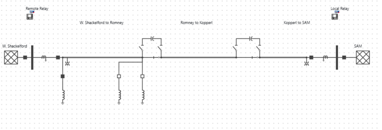
Fig. 6. Topology of Line 2 with capacitor banks and Romney shunt reactors bypassed.
