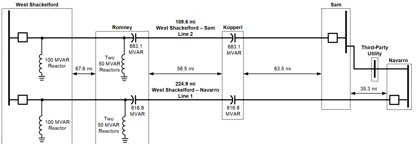
Fig. 1. Simplified one-line diagram of West Shackleford to Sam (Line 2) and West Shackleford to Navarro (Line 1) series-compensated lines.
