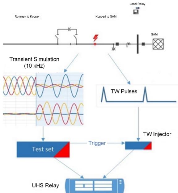
Fig. 7. TW pulses superimposed on conventional test signals [5].
