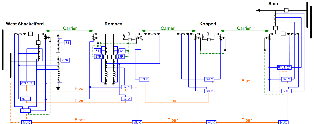
Fig. 3. West Shackleford to Sam (Line 2) one-line diagram [2].
