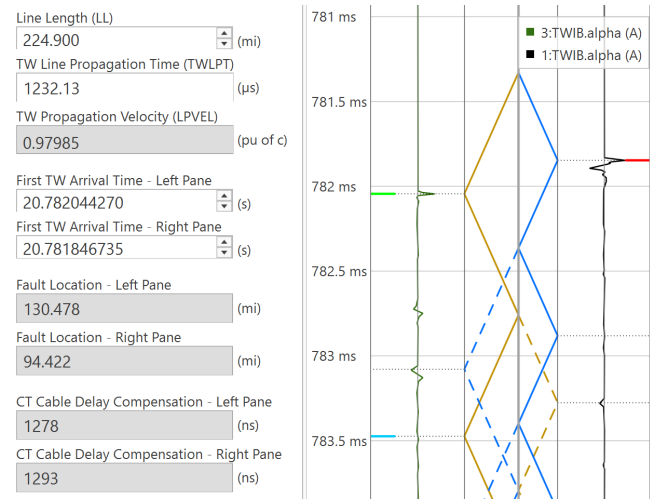
Fig. 53. Bewley diagram showing B-phase alpha-mode current TWs for both terminals.
