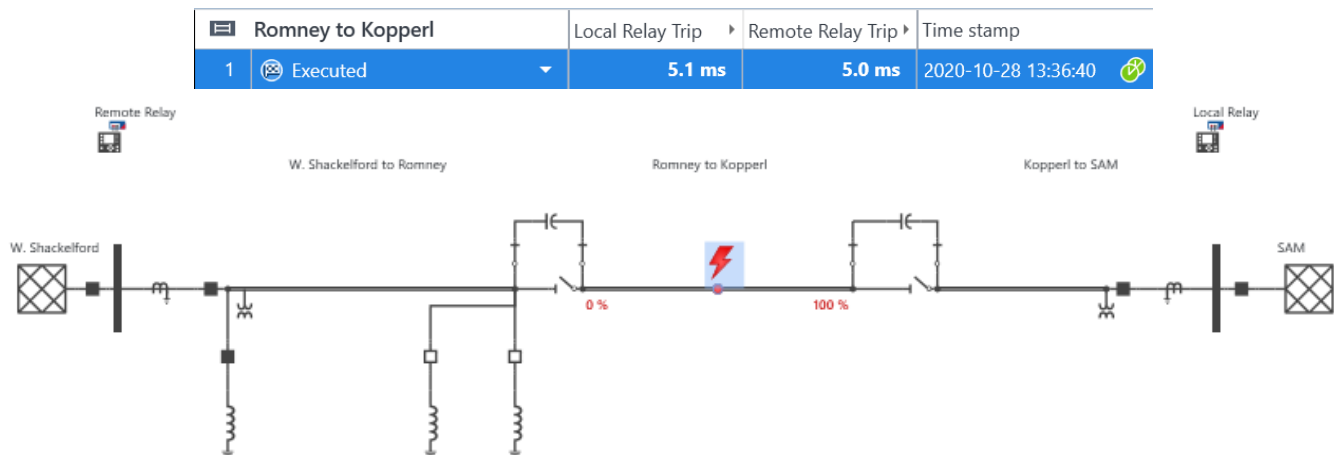
Fig. 15. Topology for the test case with a fault on the protected line with capacitor banks in service.
