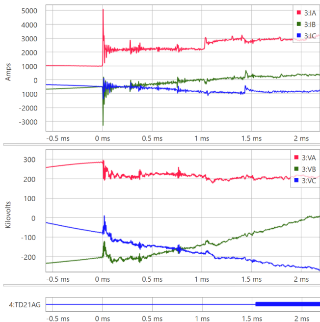
Fig. 36. West Shackleford currents and voltages and TD21AG operating time.
