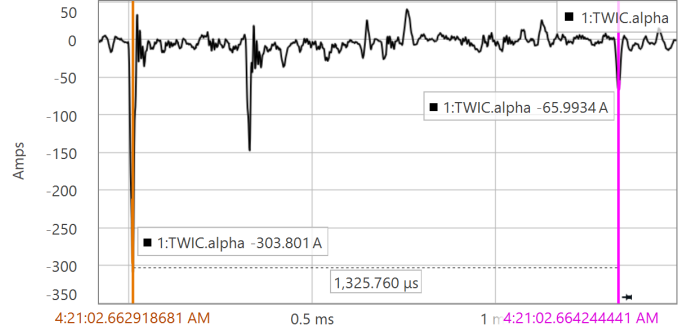
Fig. 31. Sam C-phase alpha-mode current TW arrival times: t_1 = 2.662918681 s and t_4 = 2.664244441 s.
