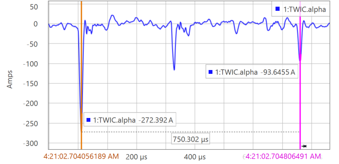
Fig. 30. West Shackelford C-phase alpha-mode current TW arrival times: t_1 = 2.704056189 s and t_4 = 2.704806491 s.
