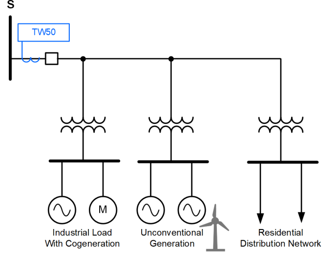
Fig. 24. Using TW50 element logic to protect tapped lines when all taps are connected through power transformers.
