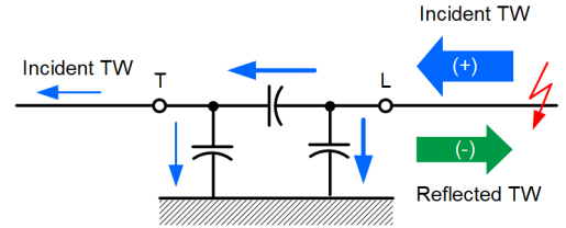
Fig. 5. TW propagation across a power transformer.
