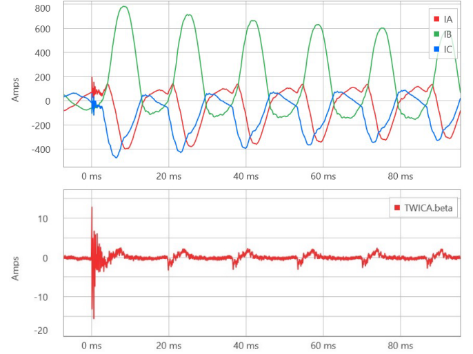
Fig. 9. Transformer inrush currents (field case).
