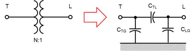
Fig. 4. Transformer representation at high frequencies.
