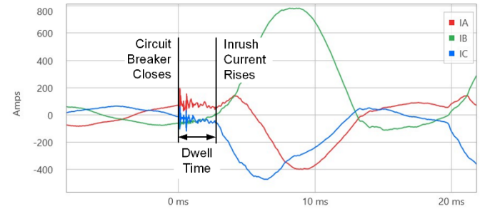
Fig. 10. Initial dwell time of about 2.8 ms.
