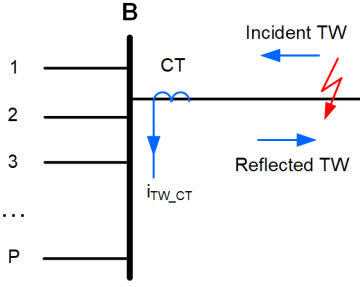
Fig. 6. Bus termination considerations.
