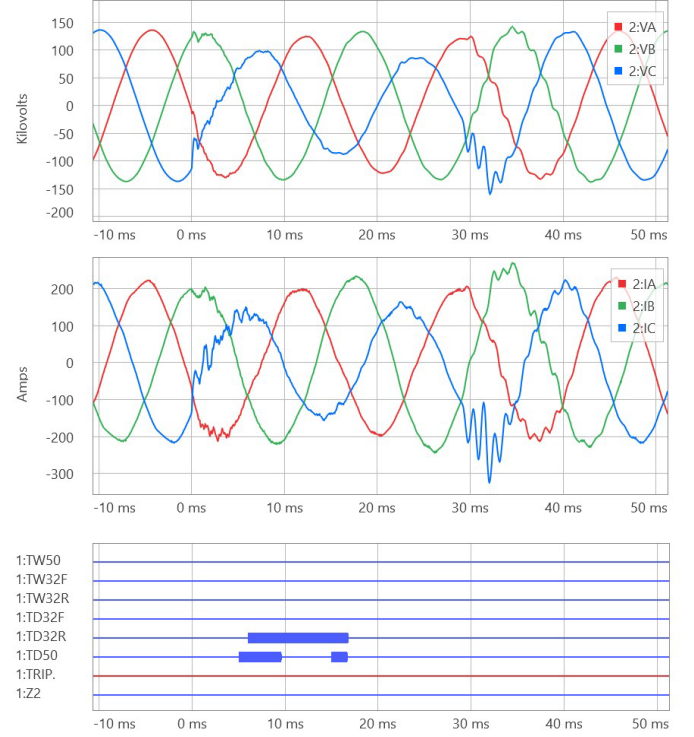
Fig. 18. Relay voltages, currents, and protection bits for a reverse fault in the grid.
