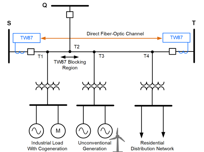
Fig. 25. Using the TW87 scheme to protect multiterminal tapped lines when taps are connected via power transformers.
