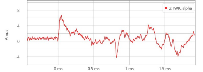
Fig. 19. Current TW for the fault quantities in Fig. 18.
