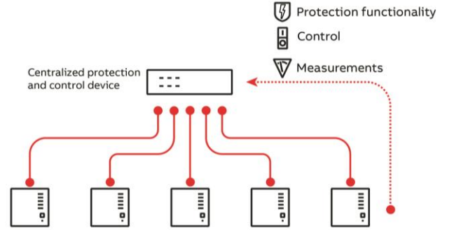
Figure 2: Simplified diagram of a CPC system
