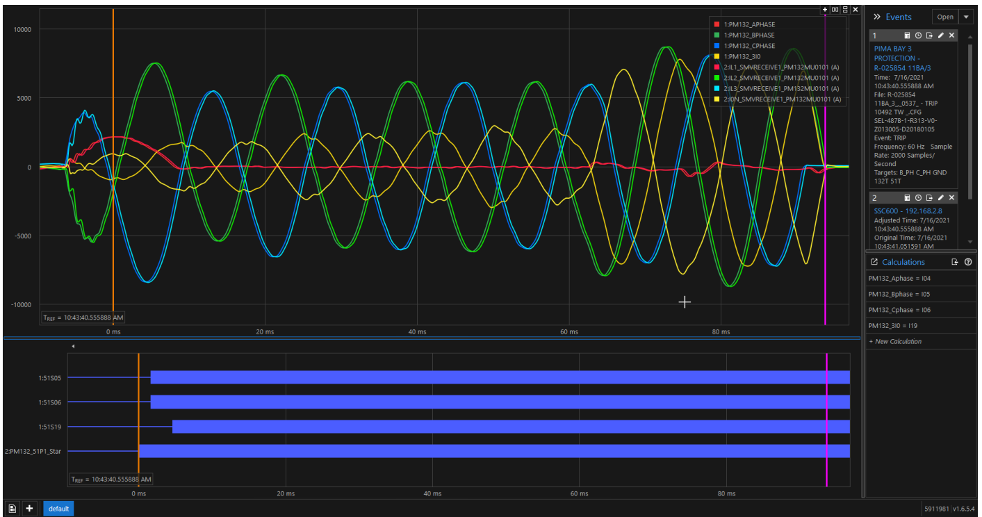
Figure 18: IPACS standard and CPC events, overlaid
