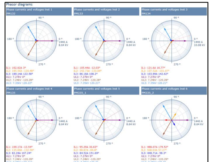
Figure 14: CPC built-in phasor diagram
