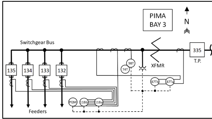
Figure 1: Existing standard PAC – 69/12.47kV Pima Substation Bay 3
