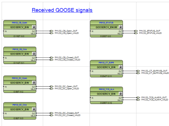
Figure 7a: GOOSE receive configuration in PM132
