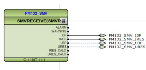
Figure 9: SMV receive function block in CPC device
