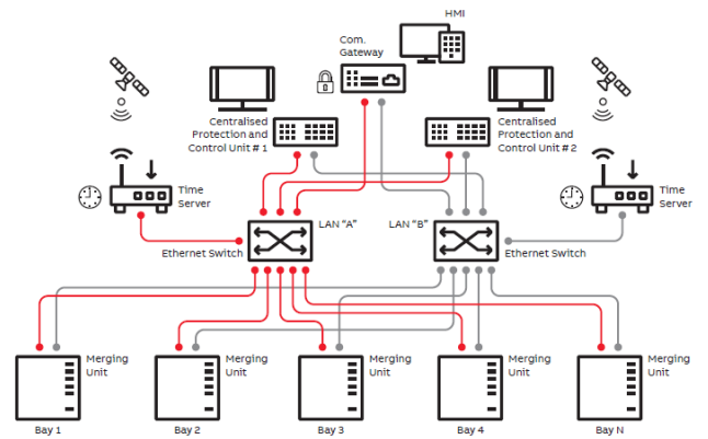
Figure 3: Redundant CPC system
