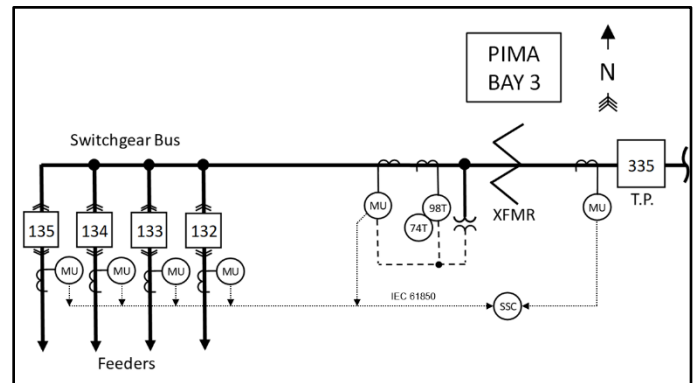
Figure 10: Pilot CPC system, non-redundant monitoring only
