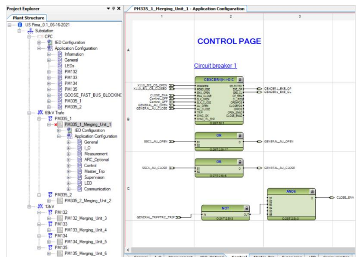
Figure 6: CB control configuration of transformer HV side MU PM335-1
