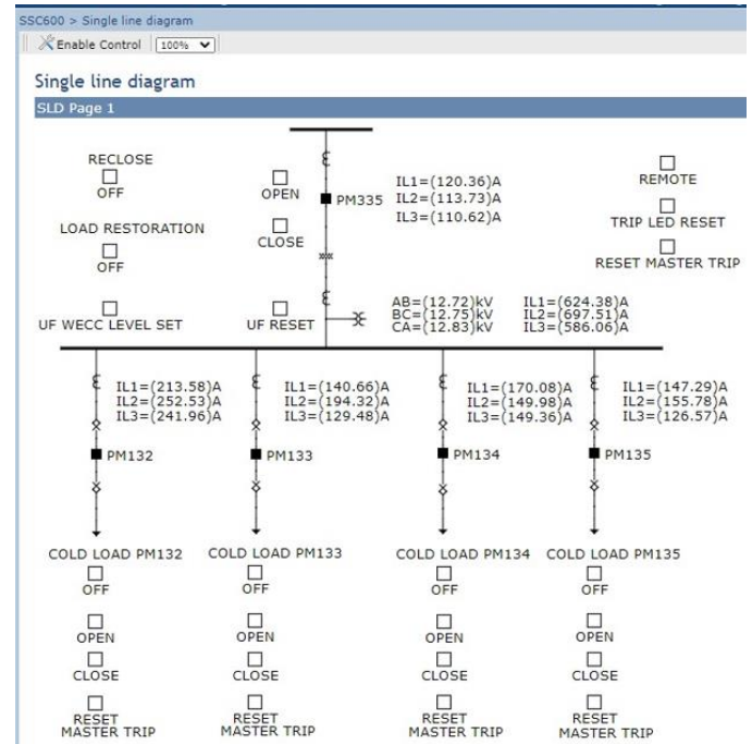
Figure 13: CPC WHMI SLD for SRP Pima Bay 3
