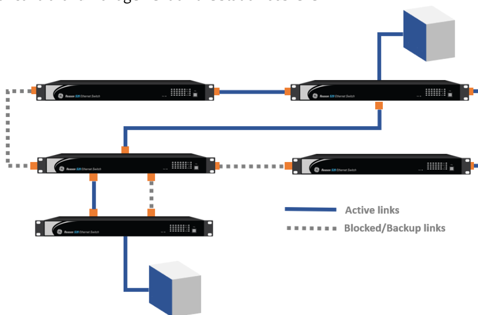
Figure 3 – Example of RSTP network topology.
