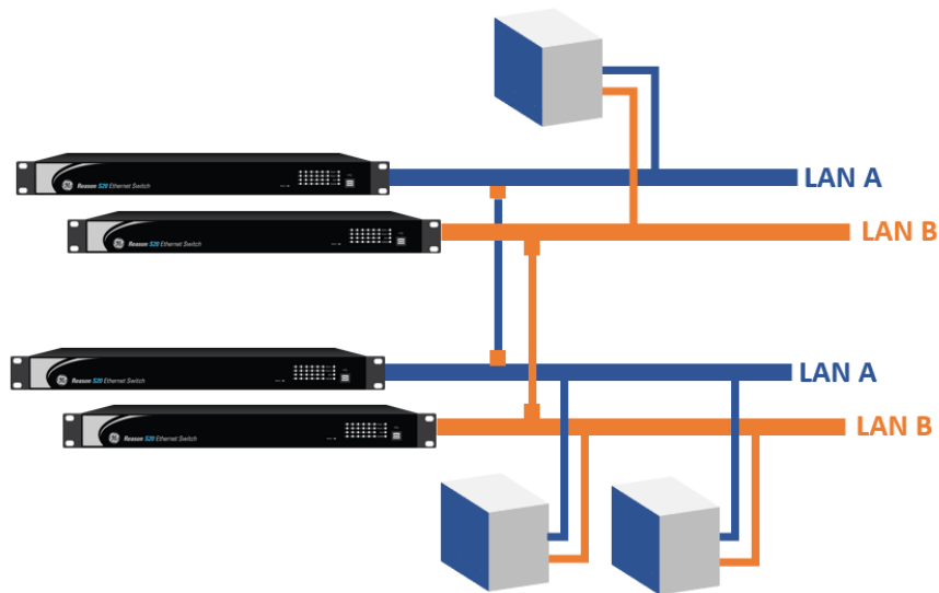
Figure 4 – Example of PRP network topology.
