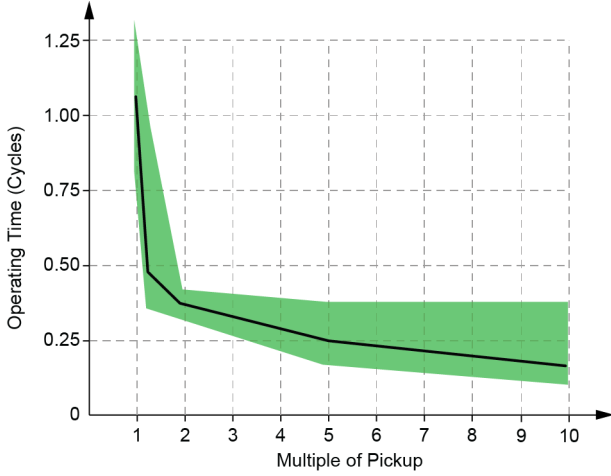
Fig. 10. Instantaneous overcurrent element operating time (range and median).
