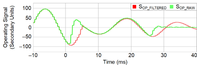
Fig. 18. Zone 1 mho raw and filtered operating signals.
