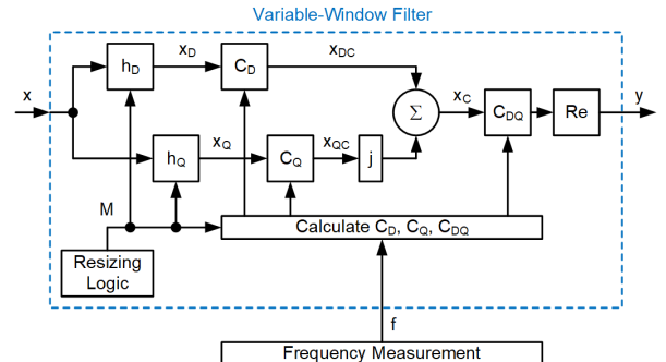
Fig. 5. Block diagram of the variable-window filter.
