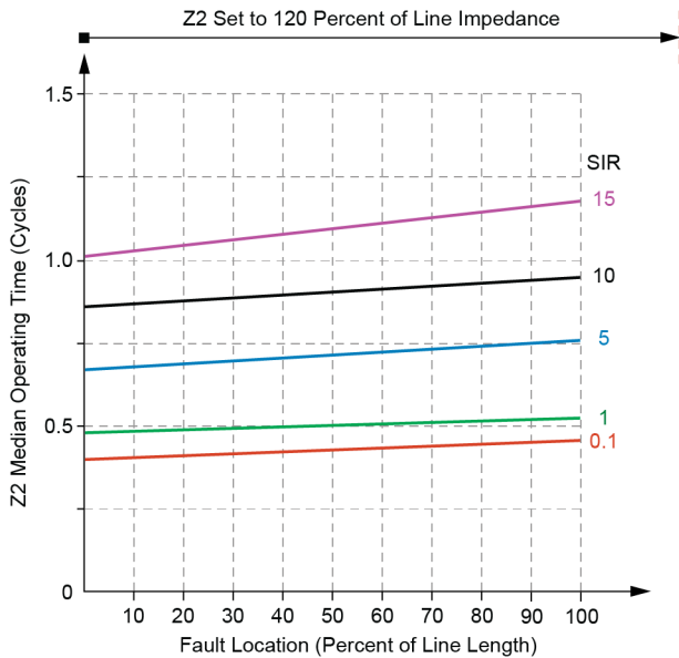
Fig. 15. Overreaching Zone 2 operating times.
