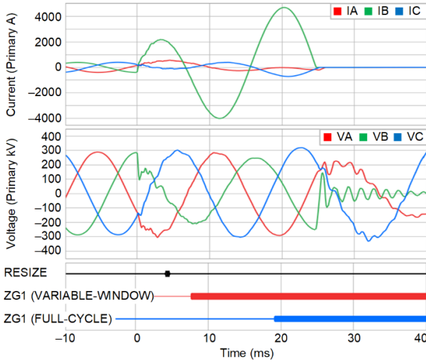
Fig. 7. Current and voltage signals during a field event.
