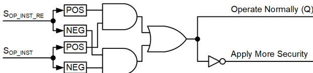
Fig. 12. Sign consistency logic checking the raw ( S_{OP\_INST} ) and filtered ( S_{OP\_INST\_RE} ) operating signals.
