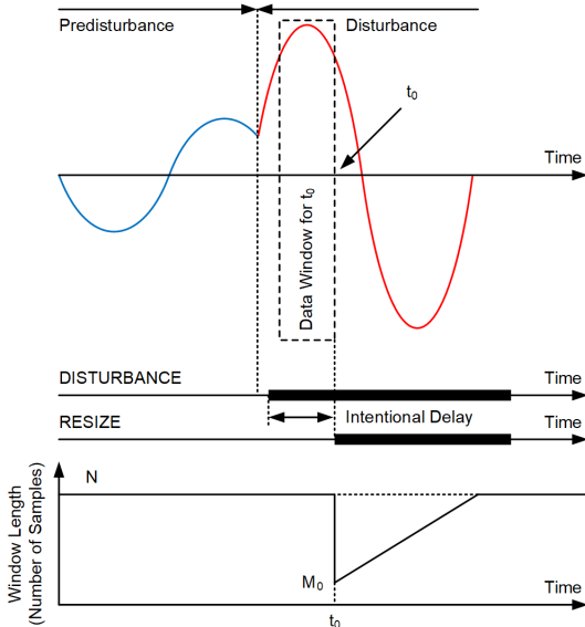
Fig. 4. Illustration of window resizing.
