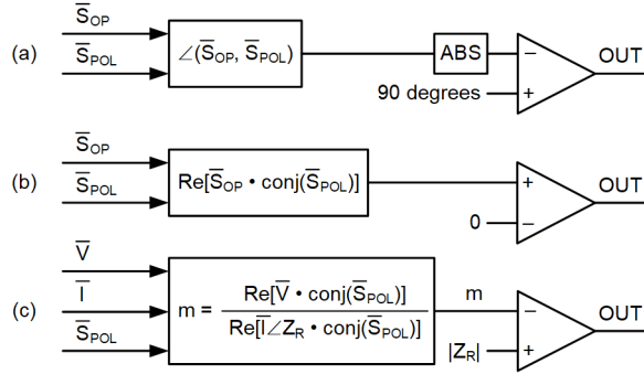
Fig. 1. Implementations of a distance comparator in phasor-based microprocessor-based relays.
