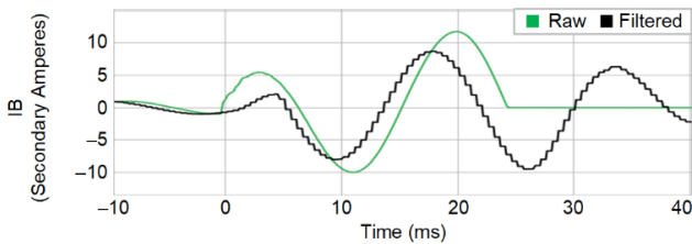
Fig. 8. Faulted phase current (raw and filtered).
