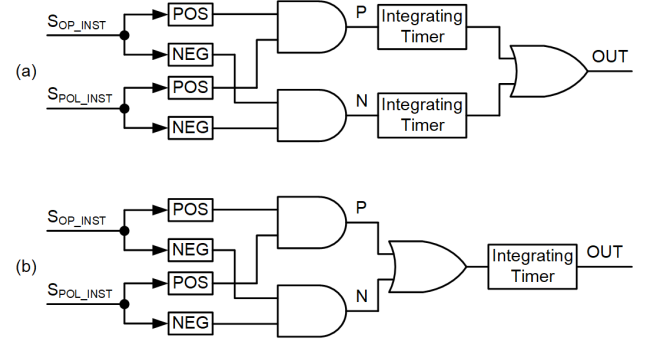
Fig. 2. Implementations of a distance comparator in static relays: (a) dual-timer method and (b) single-timer method.
