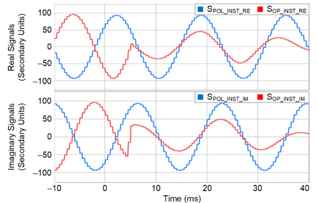
Fig. 17. Zone 1 mho operating and polarizing signals (real and imaginary parts).
