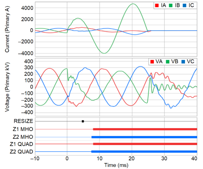
Fig. 16. Current and voltage signals during a field event.
