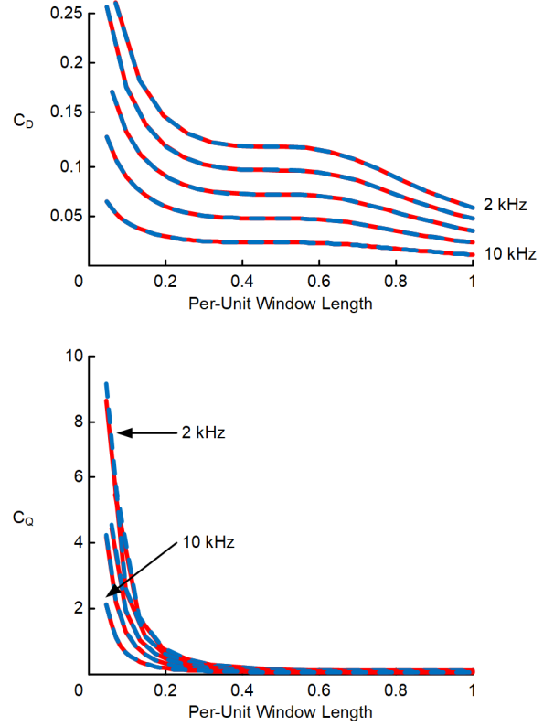
Fig. 6. Approximate (blue) and true (red) gain-correcting coefficients.
