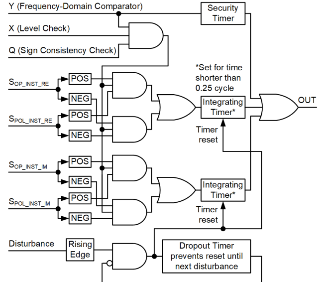
Fig. 11. New distance comparator logic diagram.
