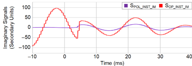
Fig. 19. Zone 1 quadrilateral operating and polarizing signals (imaginary parts).
