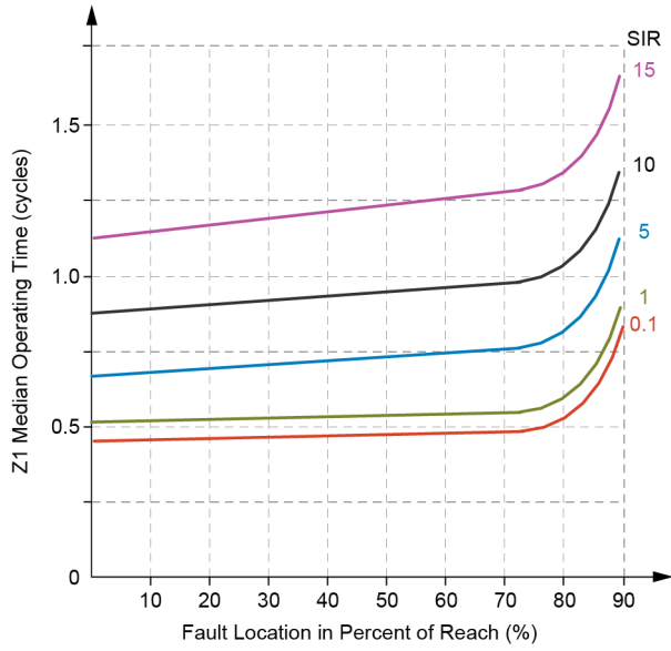
Fig. 14. Underreaching Zone 1 operating times.
