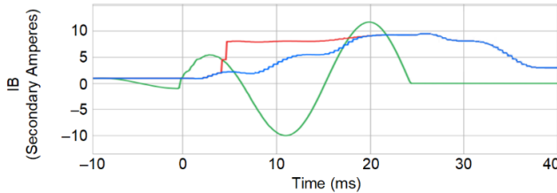
Fig. 9. Faulted phase current: raw (green) and magnitude measured with the presented method (red) and the full-cycle Fourier method (blue) for comparison.
