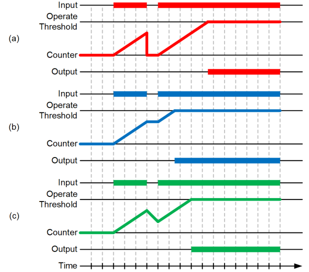
Fig. 3. Integrating timer: (a) instantaneous reset, (b) hold, and (c) integrate down.
