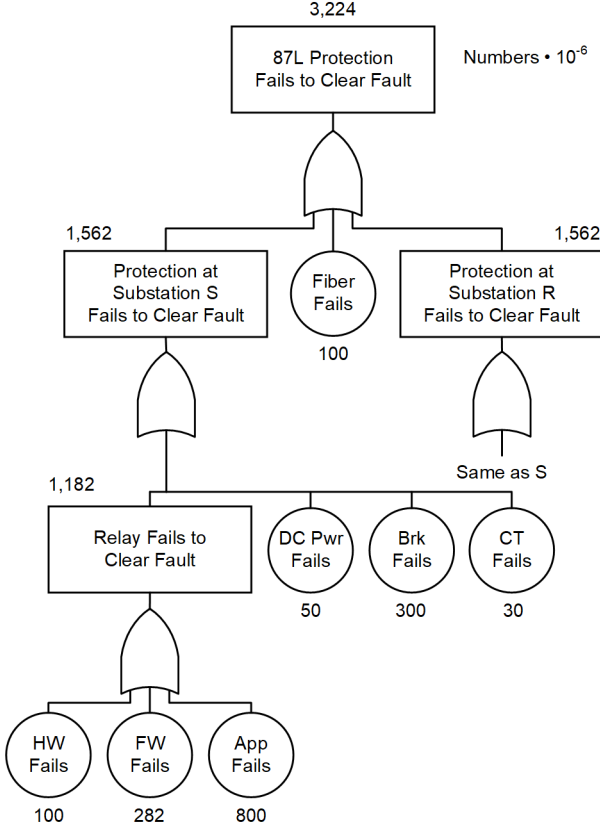
Fig. 5. System 1 Line Current Differential Protection Fault Tree Analysis
