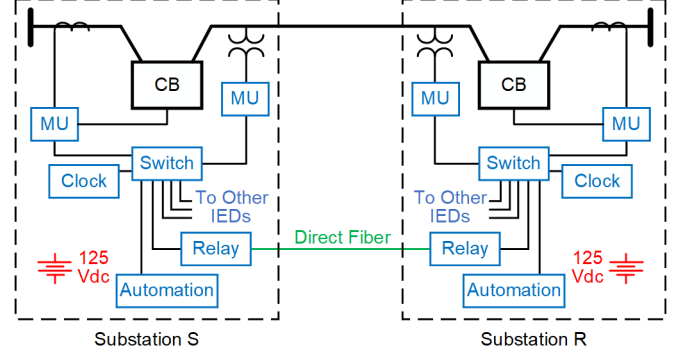
Fig. 6. System 2 Sampled Values Line Protection Substation Configuration
