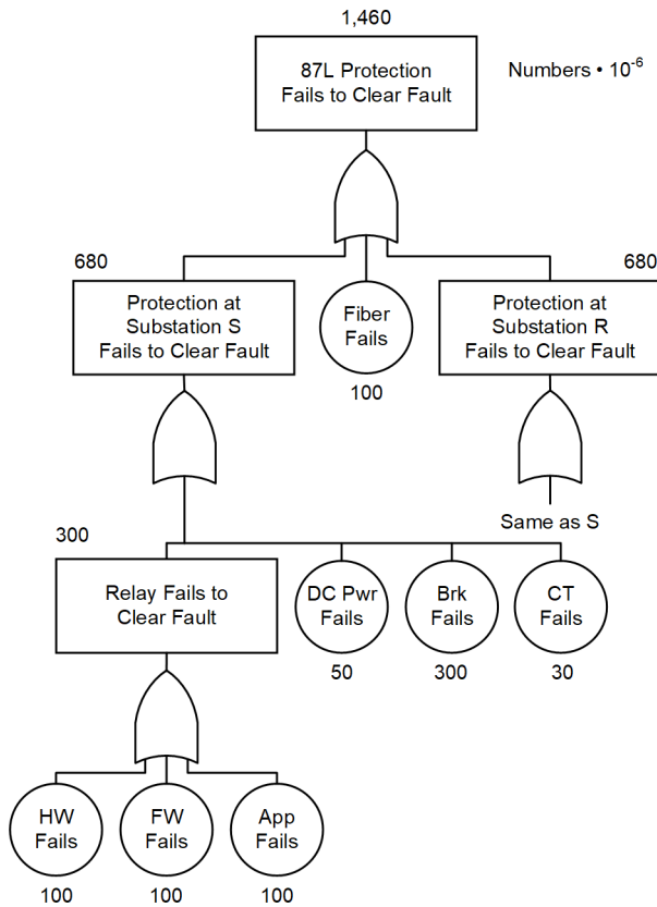
Fig. 11. Simple Line Current Differential Protection System Fault Tree Analysis
