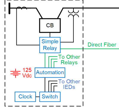
Fig. 9. Simple Protection System Substation Configuration
