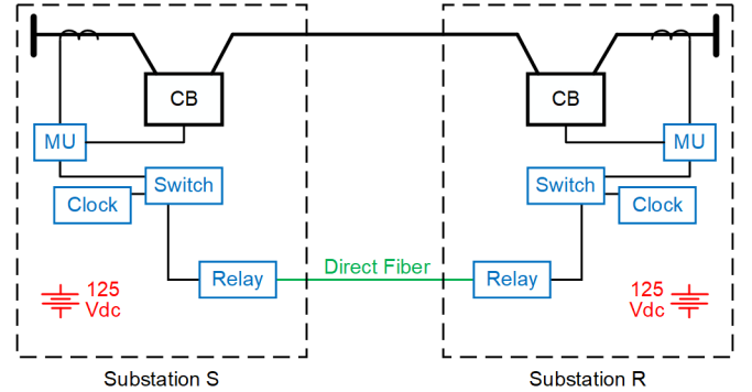
Fig. 7. System 2 Sampled Values Line Current Differential Protection Scheme
