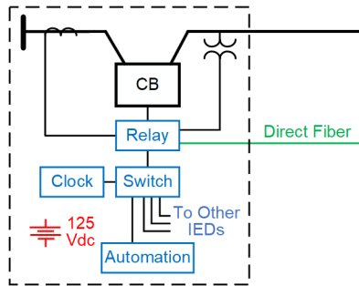
Fig. 1. Simplified Substation Protection, Automation, and Communications Diagram
