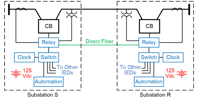
Fig. 3. System 1 Line Protection Substation Configuration
