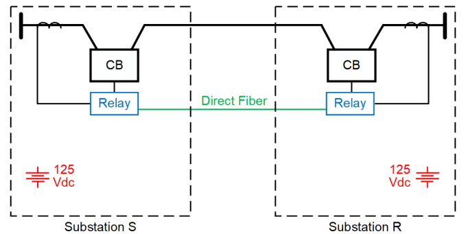
Fig. 4. Protection Elements Required to Detect and Clear a Fault
