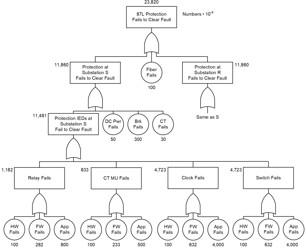
Fig. 8. System 2 Sampled Values Line Current Differential Protection Fault Tree Analysis
