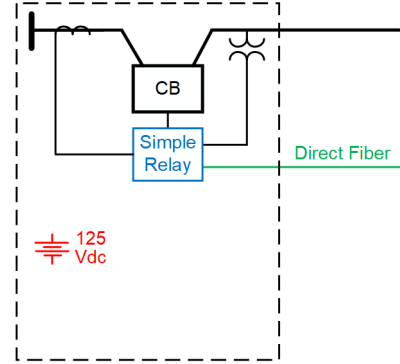
Fig. 10. Simple Protection System Elements Required to Detect and Clear a Fault
