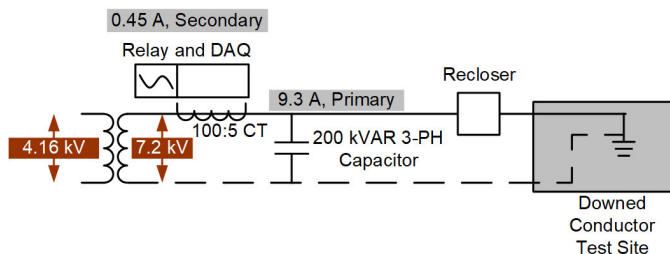
Fig. 11. Staged HIF setup included a 200 kVAR capacitor bank that provided load current that allowed the HIF algorithm to tune prior to the downed conductor testing.
