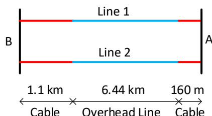
Fig. 1. Topology of the double-circuit line
