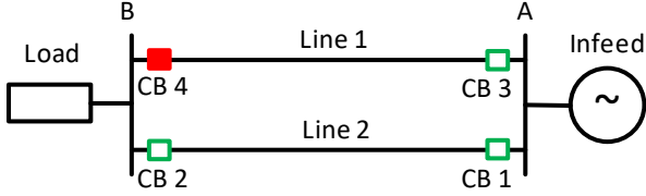
Fig. 5. Switching state 4
