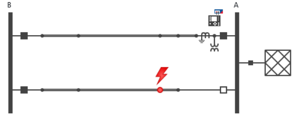
Fig. 6. Entering the line topology
